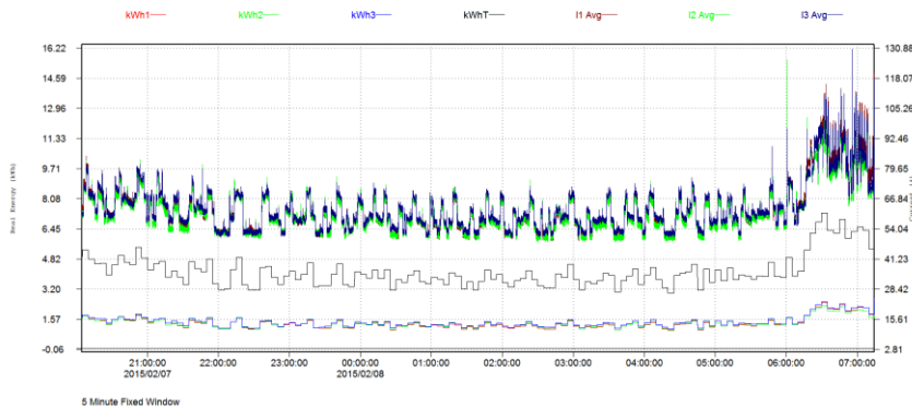
EP0002.EPF - Wh and Current Graph (Zoomed) 2015/02/07 20:04:15 to 2015/02/08 07:14:13
